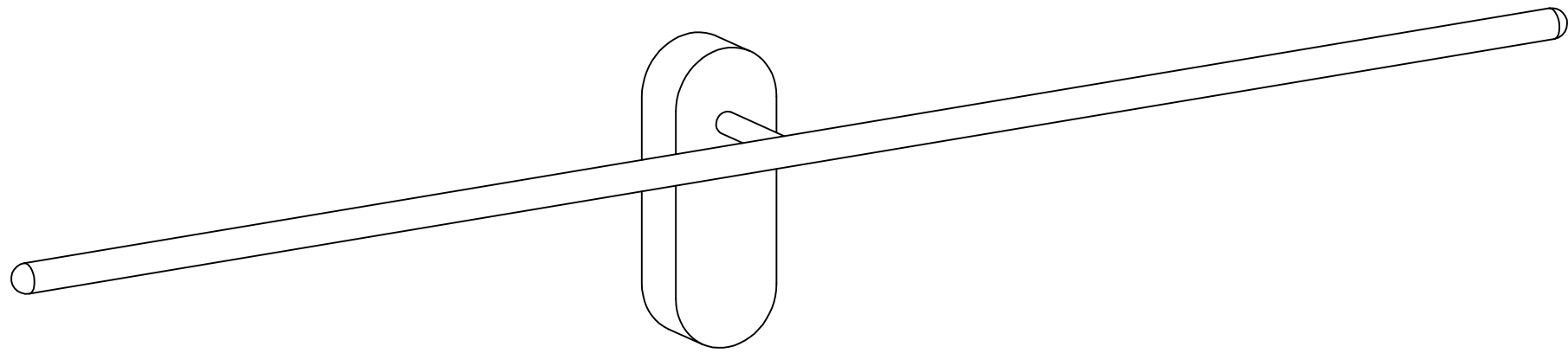
LINE 243A L900×W160×H110(mm) SMD-10W
