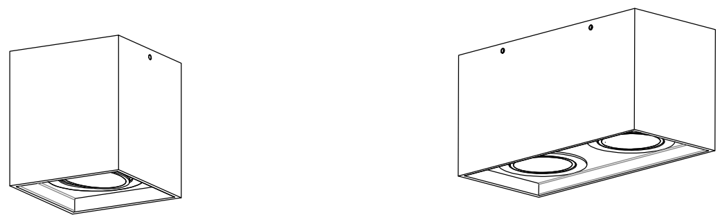
90x90x100(mm) 180x90x100(mm)
