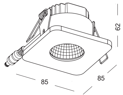
DIANA 979 GLASS
